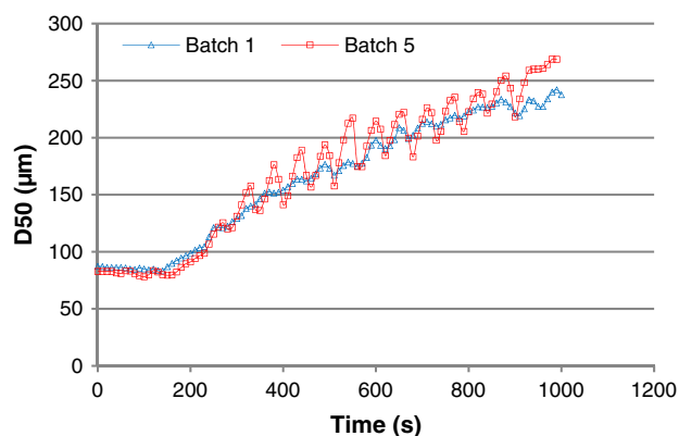
Fig. 8. In-line SFV data during spraying phase of batches 1/5 (1% HPMC, 0.2% Tween 20, 40 °C/50 °C spraying T , 50 °C drying T ).
