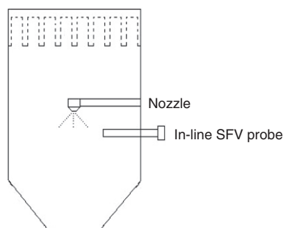
Fig. 1. Fluid bed granulator with in-line SFV probe (probe at a height of 20 cm and depth of 5 cm).
