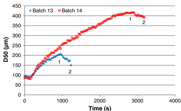
Fig. 6. In-line SFV data of batches 13/14 (1%/3% HPMC, 0.2% Tween 20, 50 °C spraying T , 70 °C drying T ) with 1: end of spraying phase and 2: end of drying phase.
