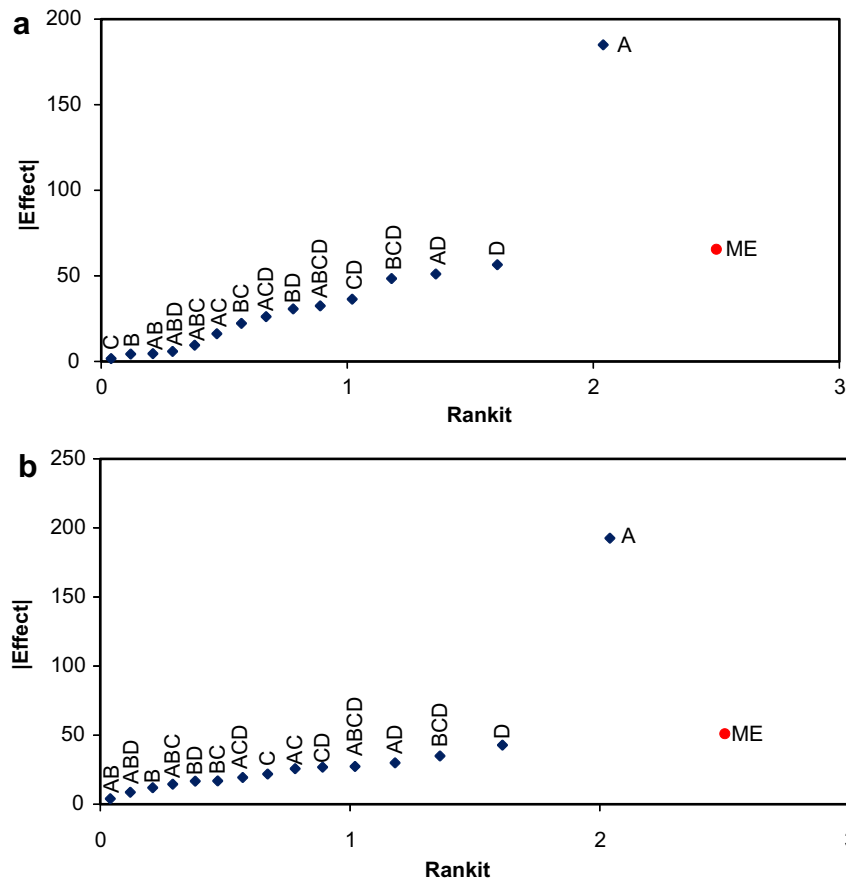
Fig. 5. Half-normal plots. (a) Half-normal plot of SFV results with critical margin of error (A = HPMC concentration, B = Tween 20 concentration, C = inlet air T during spraying, D = inlet air T during drying). (b) Half-normal plot of LD results with critical margin of error (A = HPMC concentration, B = Tween 20 concentration, C = inlet air T during spraying, D = inlet air T during drying).
