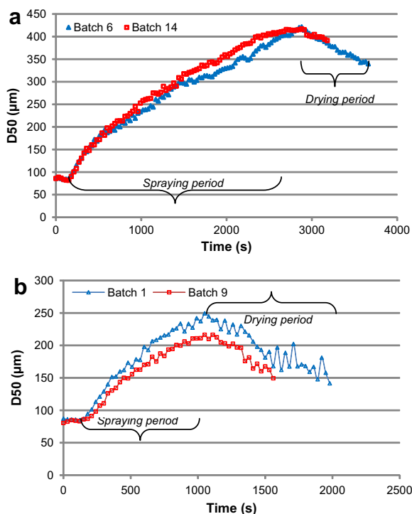
Fig. 7. In-line SFV data of batches with a different drying T . (a) In-line SFV data of batches 6/14 (3% HPMC, 0.2% Tween 20, 50 °C spraying T , 50 °C/70 °C drying T ). (b) In-line SFV data of batches 1/9 (1% HPMC, 0.2% Tween 20, 40 °C spraying T , 50 °C/70 °C drying T ).
