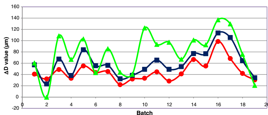
Fig. 3. Differences between the D_{10} (red circles), the D_{50} (blue squares) and the D_{90} results (green triangles) of the SFV and LD measurements for the 19 DOE batches. (For interpretation of the references to colour in this figure legend, the reader is referred to the web version of this article.)
