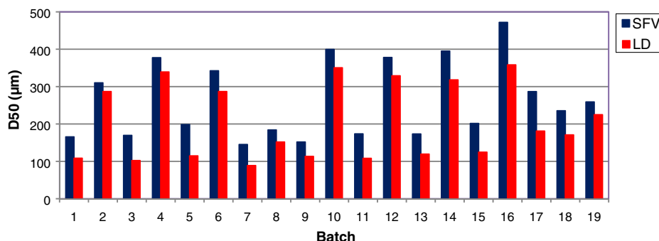
Fig. 2. Comparison between the D_{50} results obtained with in-line SFV and off-line LD for all DOE batches.
